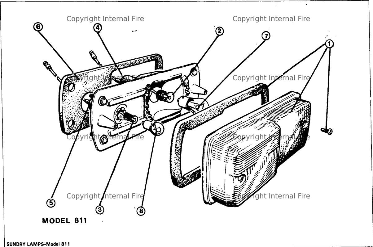
SUNDRY LAMPS-Model 811
