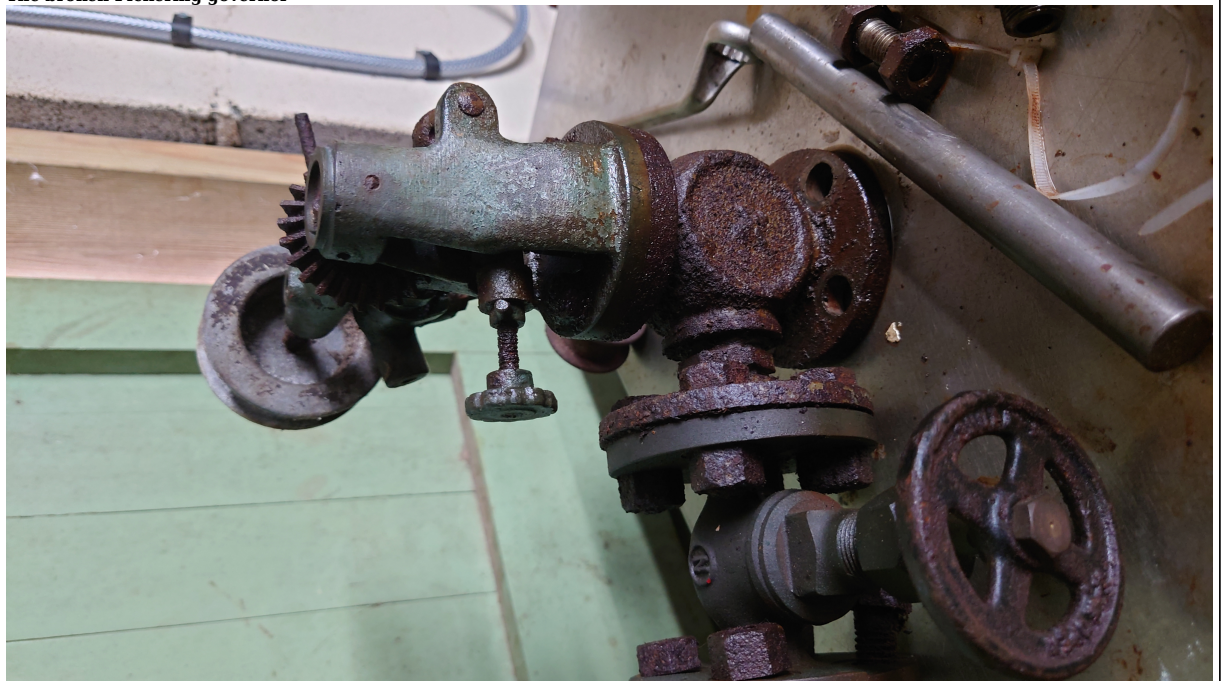
The broken Pickering governor
