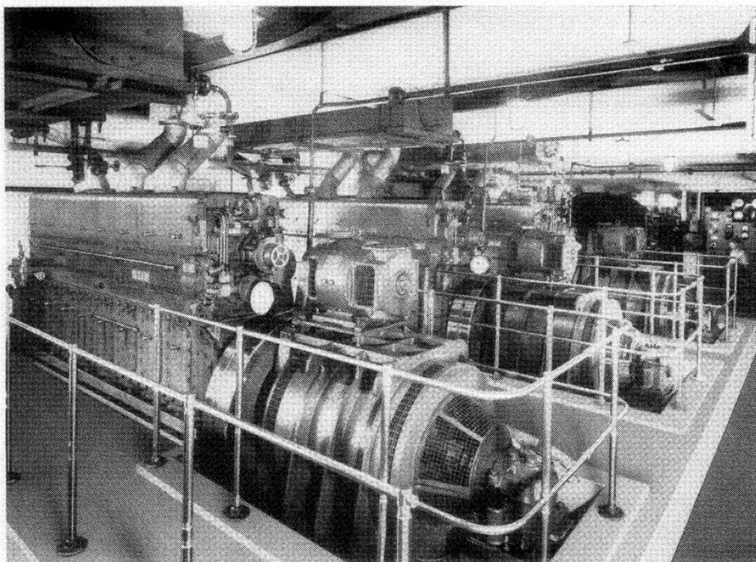
803 kW. Diesel Engine Generating Plant at the Admiralty Citadel
